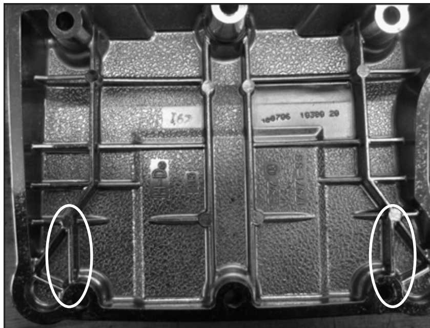
Fig. 2 Rocker cover ribs where contact can occur.
