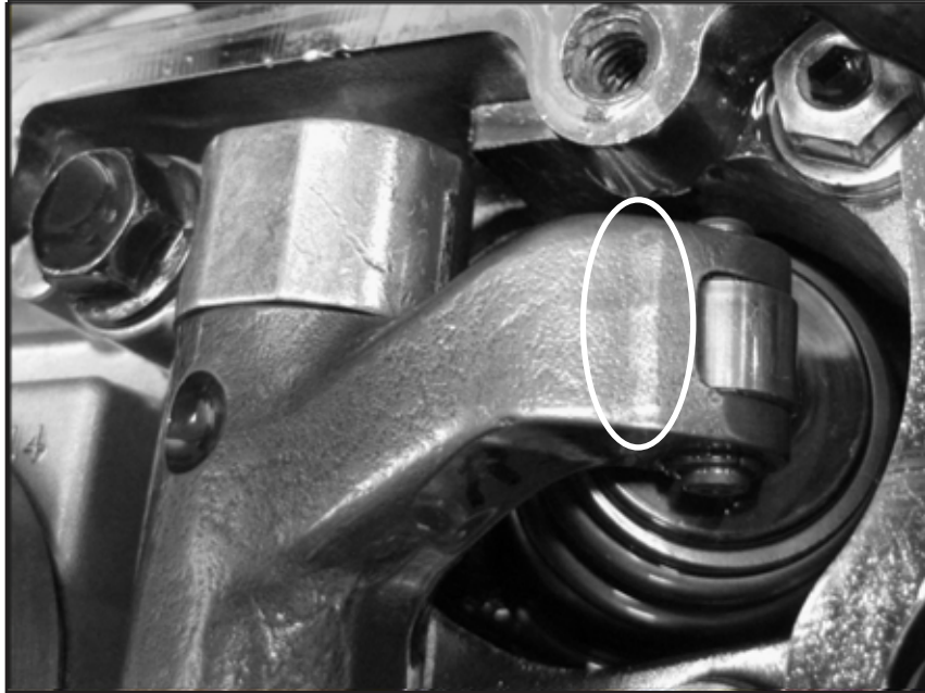
Fig. 1 Rocker arm showing contact occurring with cover rib.
